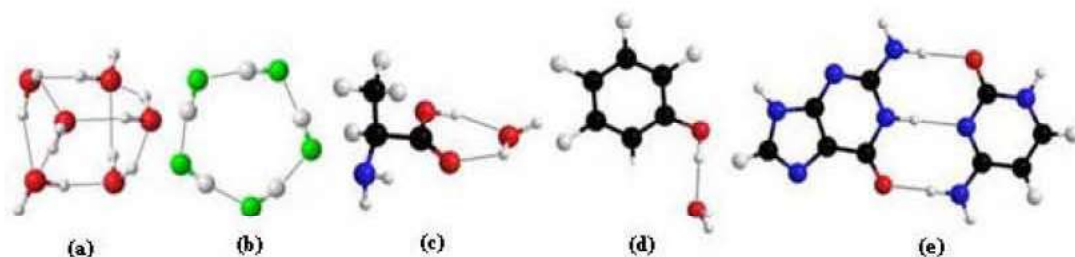
Fig. 1: Schematic view of hydrogen-bonded complexes examined in this study. Different colors are used to represent the atoms in the complex (red: oxygen, green: fluorine, blue: nitrogen, black: carbon, white: hydrogen) Dotted lines represent the hydrogen bonding in the complex. (a) water hexamer (prism configuration) (b) hydrogen fluoride pentamer (c) alanine-water complex (d) phenol-water complex (e) guanine-cytosine base pair.
