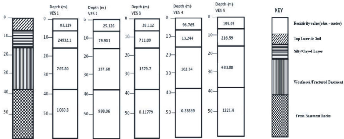
Fig. 3: Resistivity Logs of some VES Points
