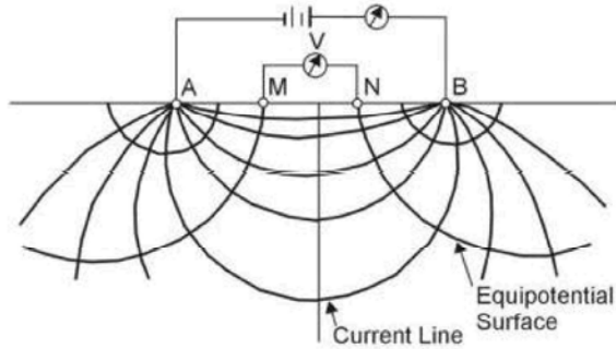
Fig. 2: Electrode configuration
