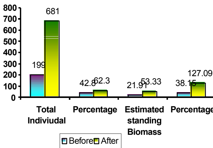
Fig. 9: Standing biomass and tree population in village agro -ecosystem of alkali affected wasteland before and after biotechnological intervention
