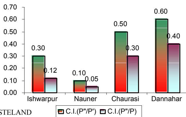
Fig. 10: Pre Existing (P), Actual P' and Potential Productivity (P'') ratings of soils under different land uses Coefficient of Improvement CI = (P''/P' and P''/P)
