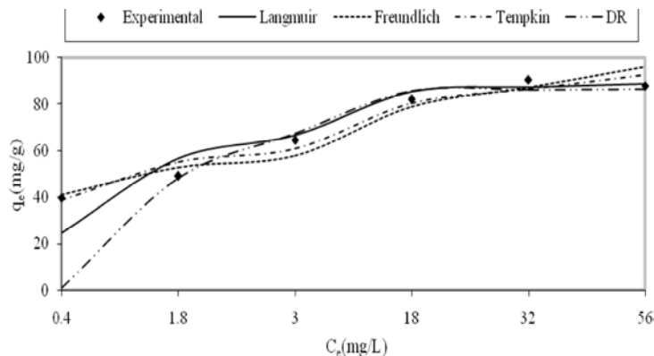
Fig. 6: a Non Linear plot of MB adsorption isotherm
