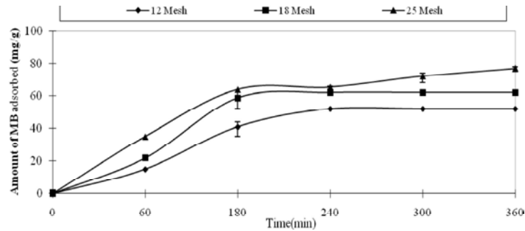
Fig. 4 a: Effect of size of adsorbent on MB adsorption Conditions: 100mL of MB solution at pH 8.5, 1g/L GAC, 130rpm shaker speed at 30°C
