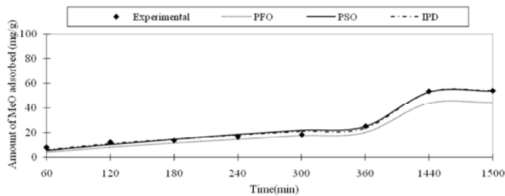
Fig. 7: b Non Linear plot of MeO adsorption kinetics
