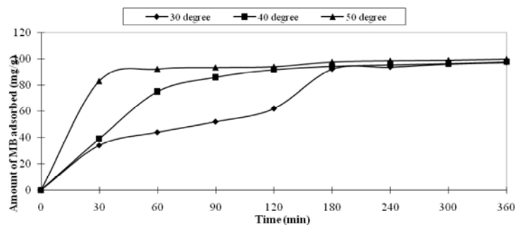
Fig. 5: a Effect of Temperature on MB adsorption Conditions: 100mL of 100mg/L MB solution at pH 8.5, 1.5 g/L of 0.088mm GAC, 250rpm shaker speed
