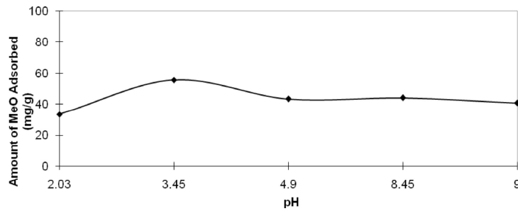
Fig. 1: b Effect of pH on MeO adsorption Conditions: 100 mL of 100 mg/L MeO solution, 1g/L of 14 mesh GAC, 130rpm shaker speed at 30°C
