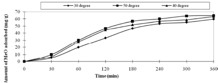
Fig. 5: b Effect of Temperature on Moe adsorption Conditions: 100mL of 100mg/L Moe solution at pH 3.5, 1.5 g/L of 0.088mm GAC, 250rpm shaker speed
