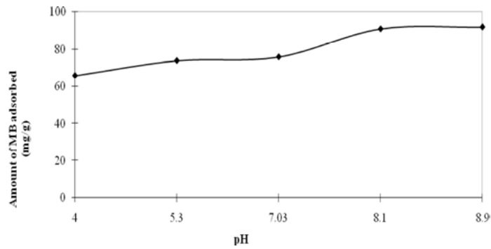
Fig. 1: a. Effect of pH on MB adsorption Conditions: 100 mL of 100 mg/L MB solution, 1g/L of 1.693 mm GAC, 130rpm shaker speed at 30°C
