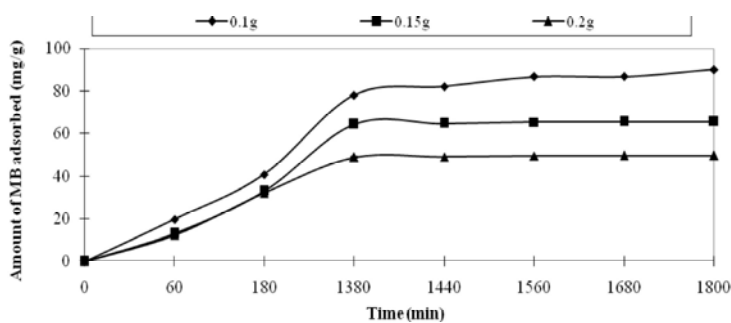
Fig. 3: a Effect of amount of adsorbent on MB adsorption Conditions: 100mL of 100 mg/L MB solution at pH 8.5, 1.698mm GAC, 130rpm shaker speed at 30°C
