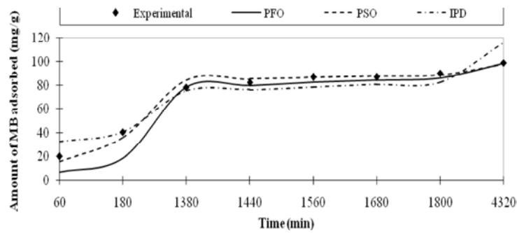
Fig. 7: a Non Linear plot of MB adsorption kinetics
