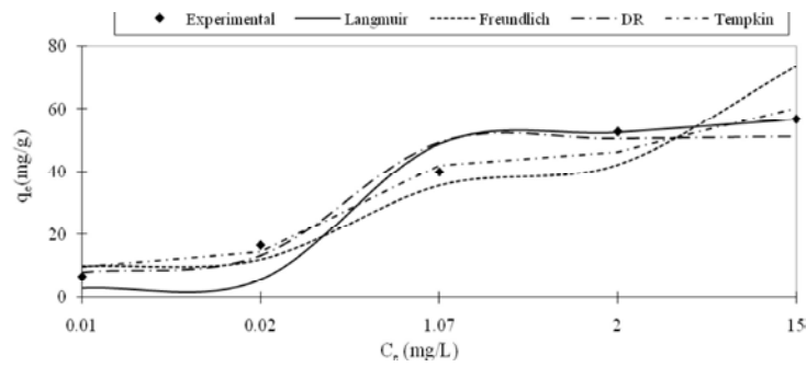
Fig. 6: b Non Linear plot of MB adsorption isotherm
