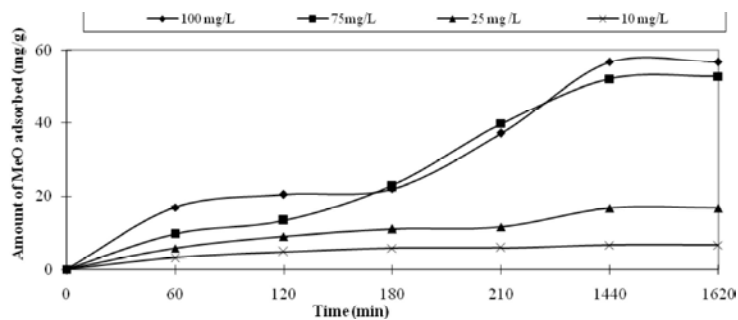
Fig. 2: b Effect of initial dye concentration on MeO adsorption Conditions: 100mL of MeO solution at pH 3.5, 1g/L of 14 mesh GAC, 130rpm shaker speed at 30°C
