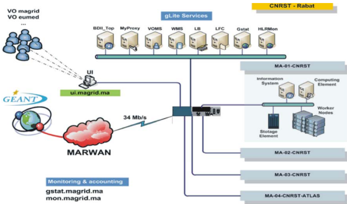
Fig. 2: Schema of Moroccan Grid Infrastructure: MaGrid
