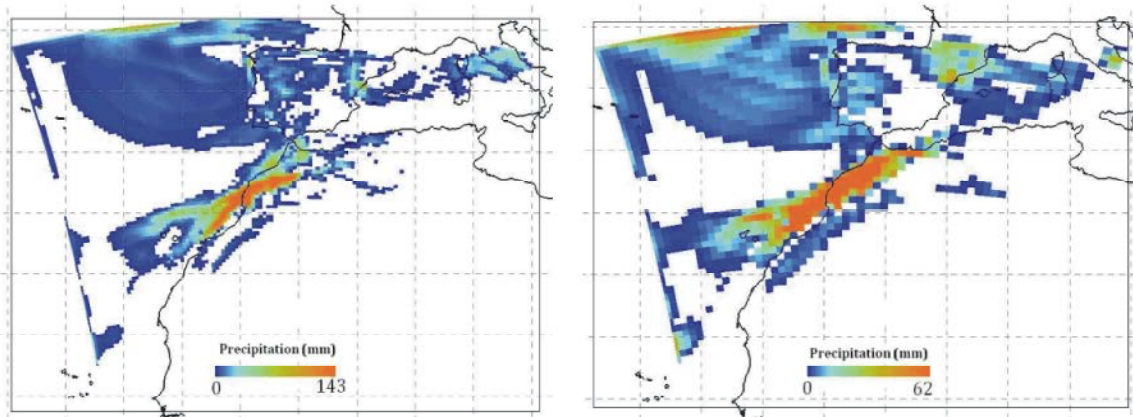
Fig. 4: Total Precipitation simulated by RegCM4.3 for 2010-11-30 with 30km (left) and 60km (right) grid spacing
