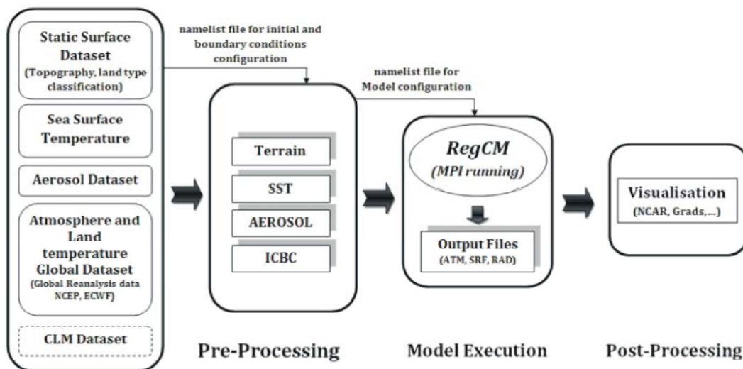
Fig. 1: RegCM4.3 workflow
