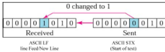
Fig. 1: Single-bit error
