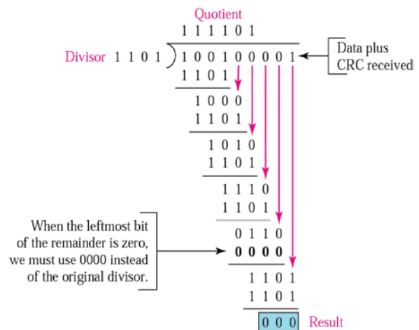
Fig. 5: CRC in receiver side
