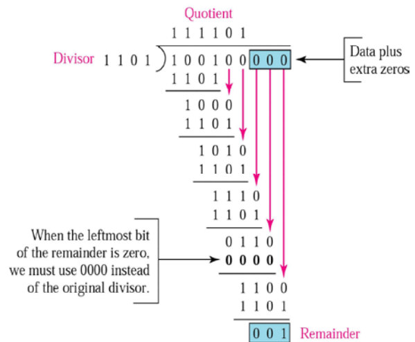
Fig. 4: CRC in sender side
