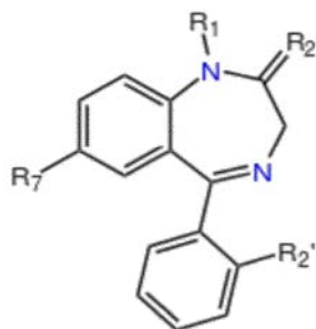
Fig. 1: Chemical structure of benzodiazepines
