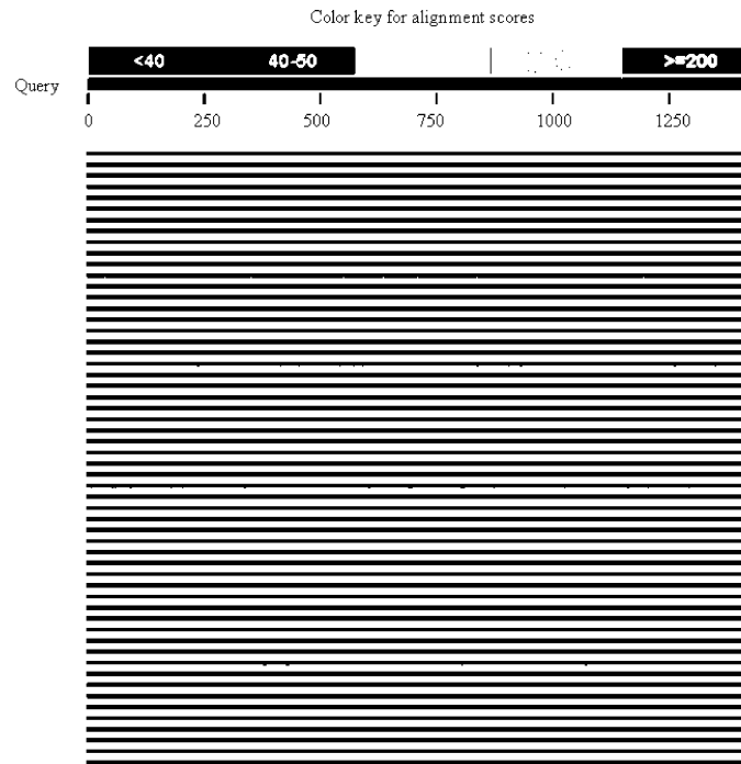
Fig. 2: BLAST DATA: (Alignment view using combination of NCBI GeneBank); Sequence Producing Significant Alignments
