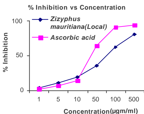
Fig. 2: Evaluation of IC_{50} of the fruit extract of Zizyphus mauritiana (Local) and standard ascorbic acid
