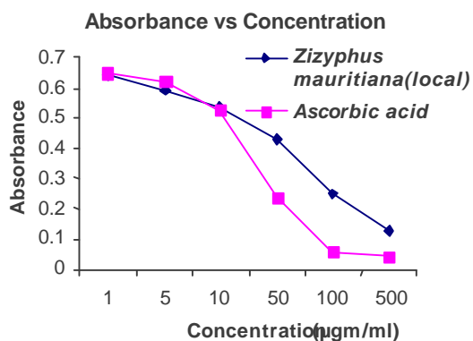
Fig. 1: DPPH scavenging Assay of the fruit extract of Zizyphus mauritiana (local) compared with standard ascorbic acid
