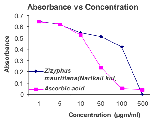
Fig. 3: DPPH scavenging assay of the fruit extract of Zizyphus mauritiana (Narikeli kul) compared with standard ascorbic acid
