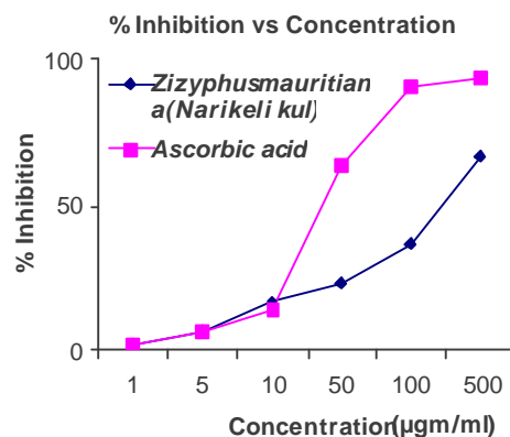
Fig. 4: Evaluation of IC_{50} of the fruit extract of Zizyphus mauritiana (Narikeli kul) and standard ascorbic acid
