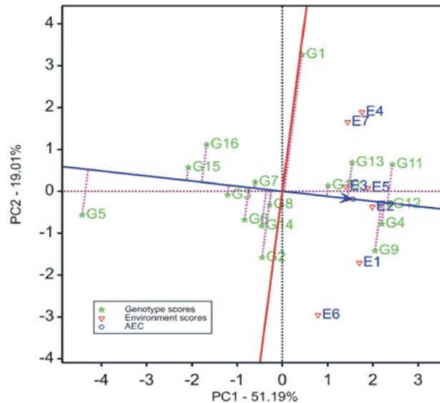
Fig. 4: GGE biplot showing grain yield rank and stability of 16 lowland rice genotypes across seven environments. E1: Woreta2014, E2: Jimma 2014, E3: Assosa2014, E4: Woreta2015, E5: Kokit2015, E6: Jimma2015, E7: Gojeb2015.
