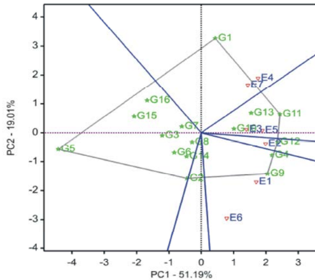
Fig. 3: GGE biplot showing winner genotypes at specific environments. E1: Woreta2014, E2: Jimma 2014, E3: Assosa2014, E4: Woreta2015, E5: Kokit2015, E6: Jimma2015, E7: Gojeb2015
