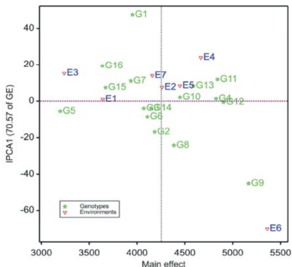
Fig. 1: AMMI1 biplot showing the main effect vs. stability (IPCA1) of both genotypes and environments on grain yield (kg ha^{-1} ). E1: Woreta2014, E2: Jimma 2014, E3: Assosa2014, E4: Woreta2015, E5: Kokit2015, E6: Jimma2015, E7: Gojeb2015.
