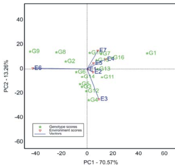
Fig. 2: AMMI 2 biplot graph showing interaction of PC1 and PC2 scores of 16 rice genotypes at seven environments. E1: Woreta2014, E2: Jimma 2014, E3: Assosa2014, E4: Woreta2015, E5: Kokit2015, E6: Jimma2015, E7: Gojeb2015.
