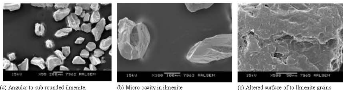
Fig. 3: SEM photo of ilmenite from northern sector
