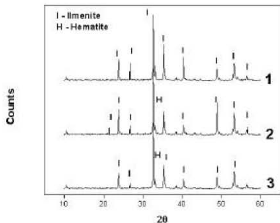
Fig. 2: X-Ray diffractograms of representative ilmenite from northern sector.
