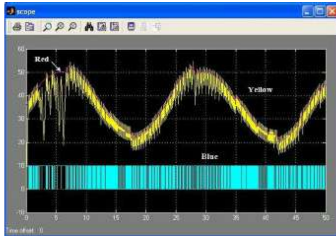
Fig. 8: Simulation results of on/off controller system with \pm 2 hysteresis value
