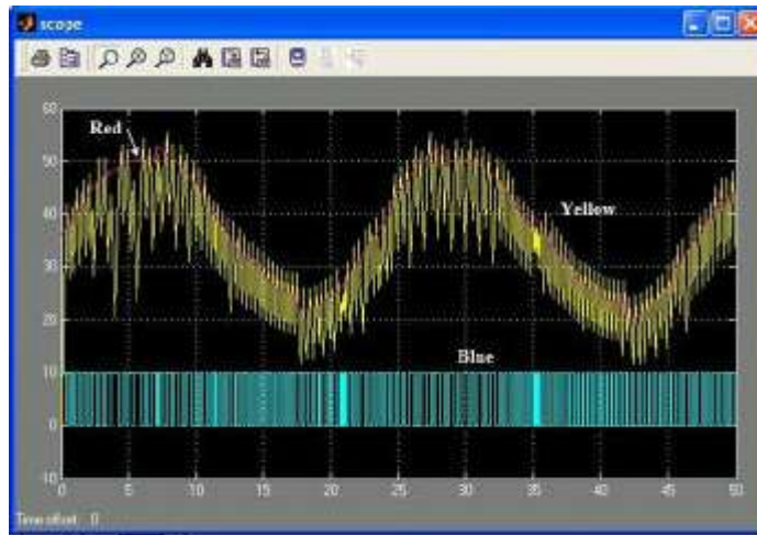
Fig. 7: Simulation results of on/off controller system with \pm 4 hysteresis value
