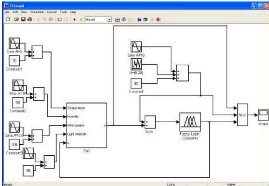
Fig. 4: Diagram of the fuzzy controller system with the soil model
