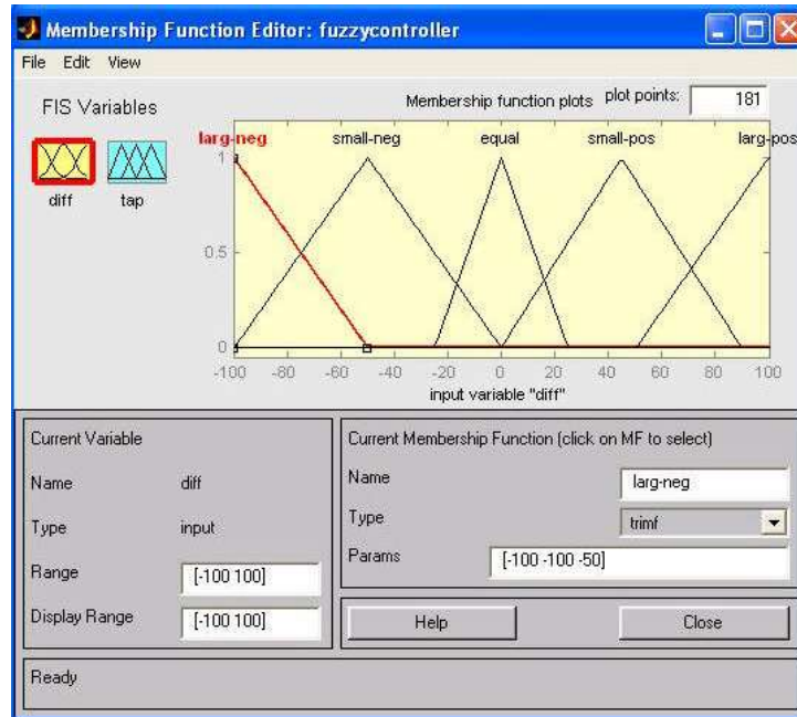
Fig. 5: Fuzzy variable "the difference between the desired and actual soil moisture values"
