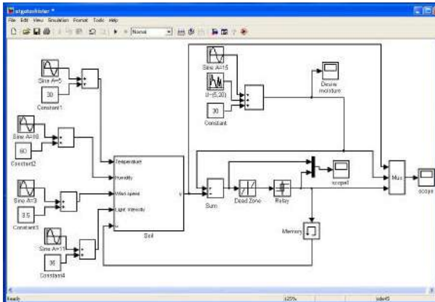
Fig. 6: Diagram of the on/off controller system with hysteresis and without it
