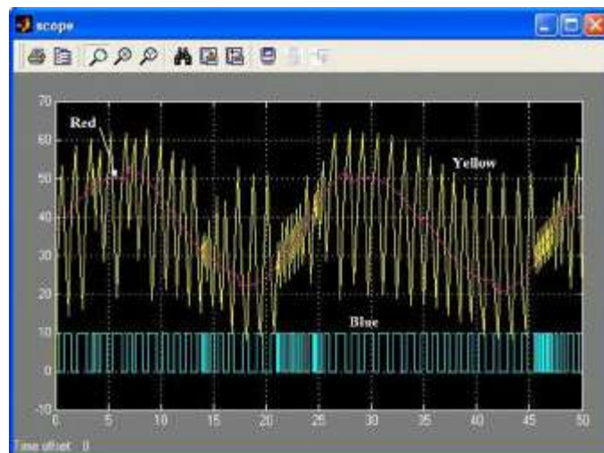
Fig. 9: Simulation results of on/off controller system without hysteresis
