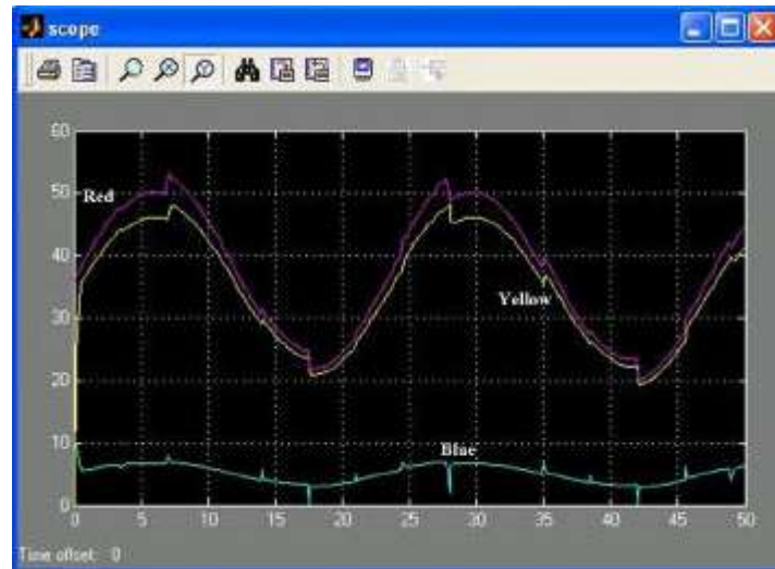
Fig. 10: Simulation results of fuzzy controller system
