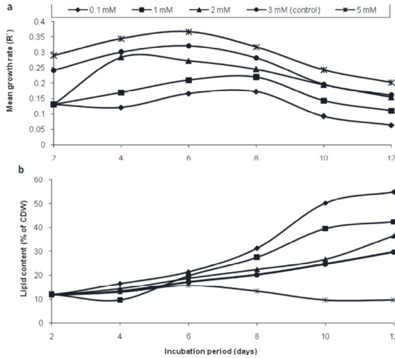
Fig. 1: Effect of different concentrations of NaNO 3 on growth (a) and lipid content (b) of C. vulgaris and cultivated for 12 days in bold basal medium.
