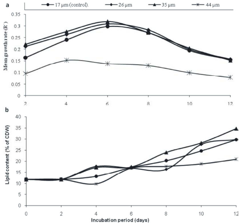
Fig. 3: Effect of different concentrations of \text{FeSO}_4 \cdot 7\text{H}_2\text{O} on growth (a) and lipid content (b) of C. vulgaris cultivated for 12 days in bold basal medium.
