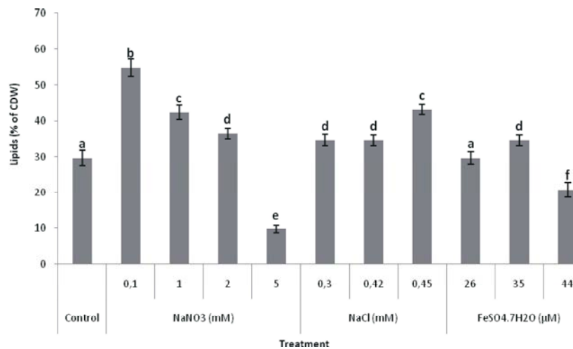
Fig. 4: Effect of nitrogen deficiency, salinity and iron concentration on lipid content of C. vulgaris (as % of CDW). Lipids were measured gravimetrically after 12 days of incubation. Error bars represent the SD from three replicates. Columns with the same letters showed insignificant difference at P = 0.05
