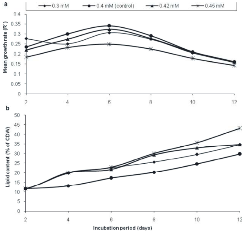
Fig. 2: Effect of different concentrations of NaCl on growth (a) and lipid content (b) of C. vulgaris cultivated for 12 days in bold basal medium.
