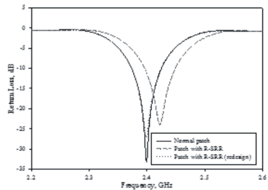
Fig. 6: Return loss of Single R-SRR antenna
