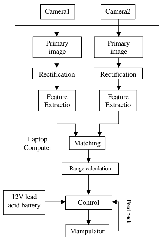
Fig. 5: Block diagram of the harvester
