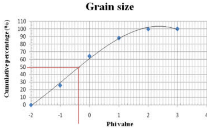
Fig. 1.1: Soil grain size graph obtained through the calculations in sieving analysis
