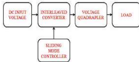
Fig. 5: Control block diagram
