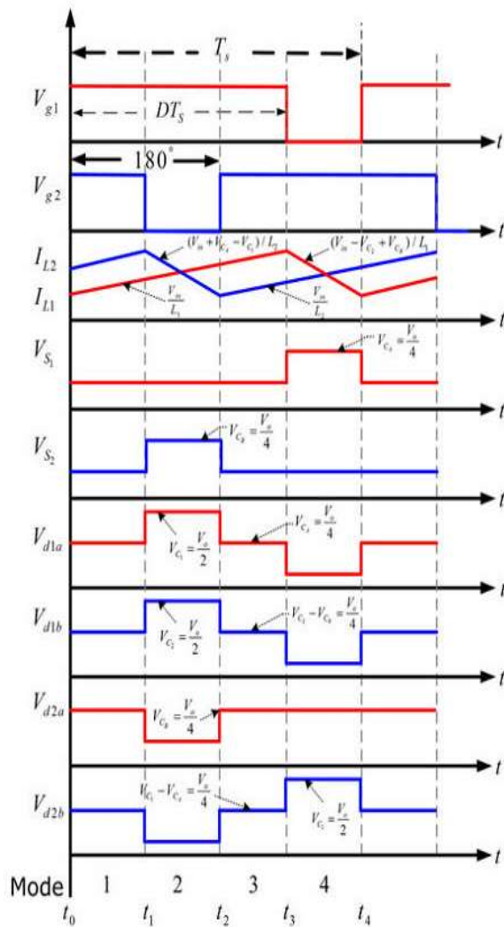
Fig. 3: Operating waveform
