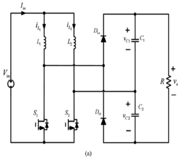
Fig. 2(a): Configuration of two-phase interleaved boost converter
