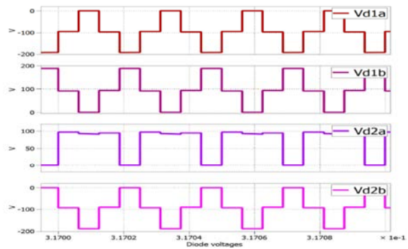
Fig. 7: Simulation result of diode voltage
