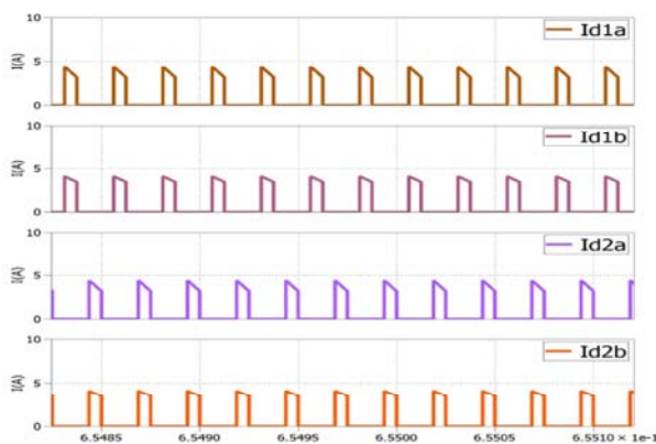
Fig. 6: Simulation result of diode current
