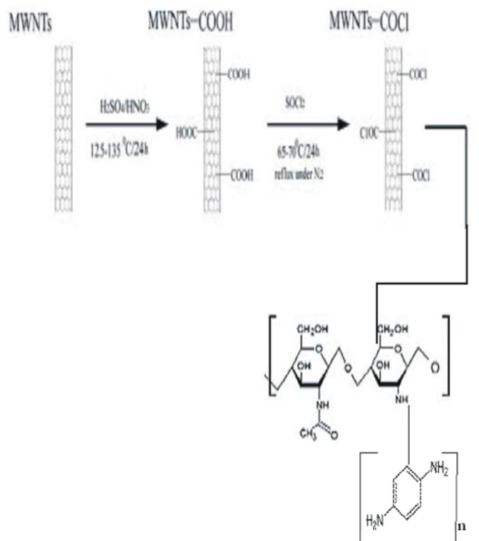
Fig. 1: Structure of Paraphenyldiamine/C-MWCNT
