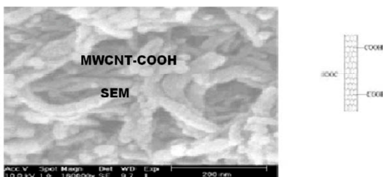
Fig. 5: SEM MICROGRAPH OF MWCNT-COOH
