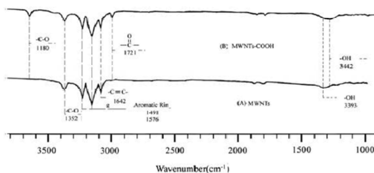
Fig. 2: FTIR spectrum of (A) MWCNT & (B) MWCNT-COOH
