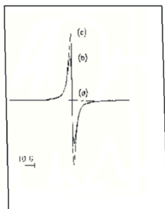
Fig. 13: Epr Spectrum of Poly (PARAPHENYLEDIAMINE)
