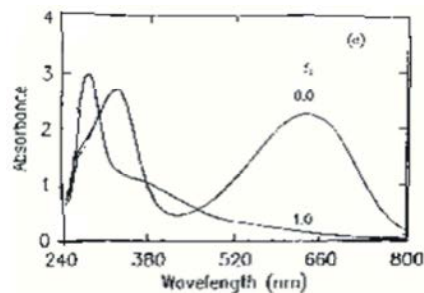
Fig. 11: UV-VIS SPECTRUM OF POLY (PARAPHENYLEDIAMINE)/C-MWCNT
