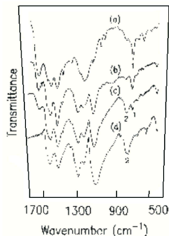
Fig. 12: FTIR SPECTRUM OF POLY (PARAPHENYLEDIAMINE)/C-MWCNT
