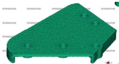
Fig. 2: Meshed Model
