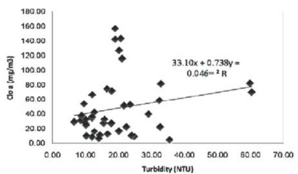
Fig. 3: Correlation between chlorophyll-a concentration and turbidity in the whole period
