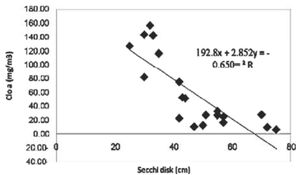
Fig. 2: Correlation between chlorophyll-a concentration and Secchi disk depth in autumn
