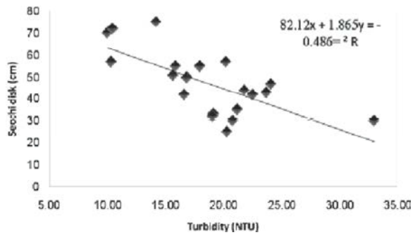
Fig. 4: Correlation between Secchi disk depth and turbidity in autumn
