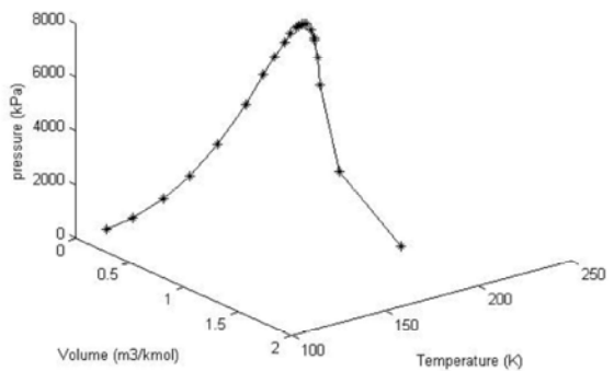
Fig. 7: PVT diagram for liquefaction cycle
