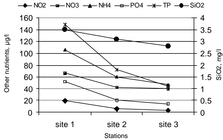
Fig. 1: Different nutrient concentrations at different sites
