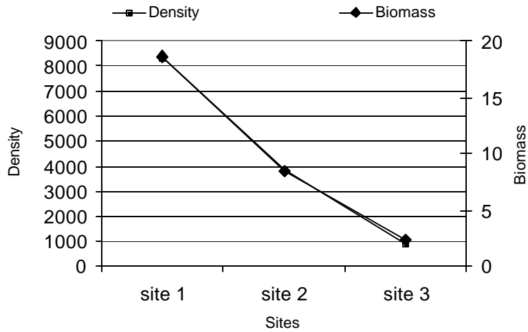
Fig. 2: Phytoplankton population density (no of cells x 10 3 /l) biomass (µg / l)
