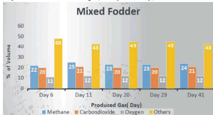
Fig. 7: Produced Gas Composition from Mixed Fodder (6 th Day - 41 th Day)
