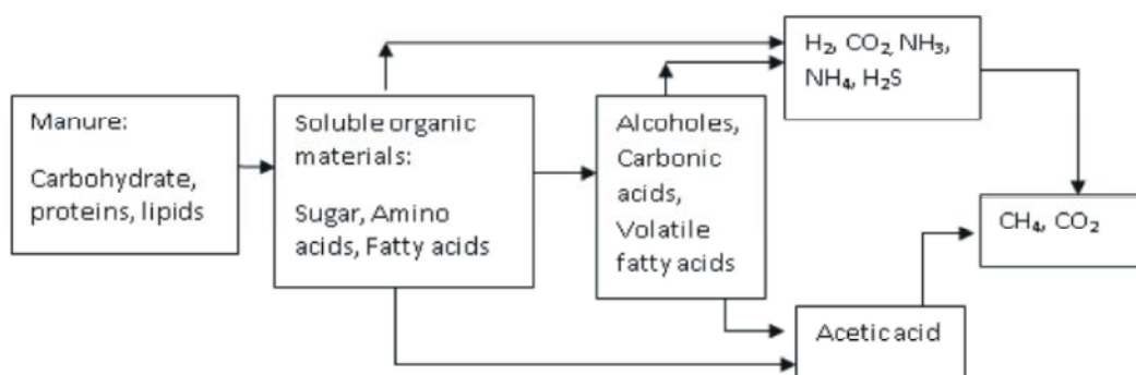
Fig. 2: Schematic diagram of anaerobic digestion
